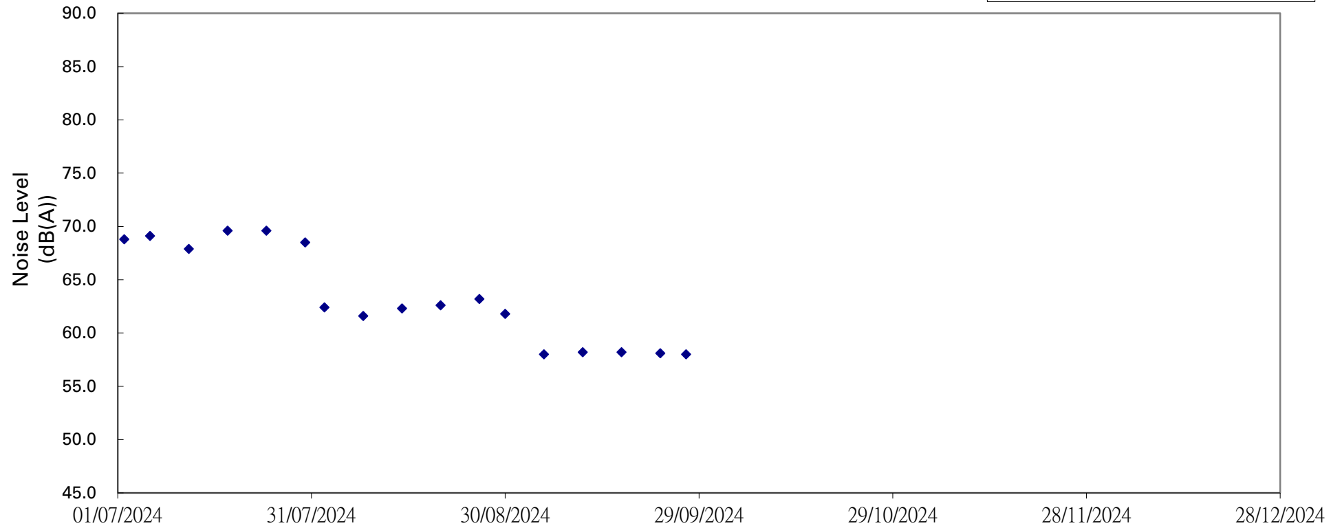
Noise Level (Leq 30 mins) dB(A) Vs Date for Location W-N1A
